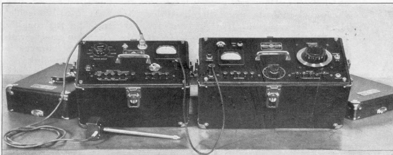
FIGURE 25. The TYPE 762-A Vibration Analyzer was designed particularly for use with the TYPE 761-A Vibration Meter.
