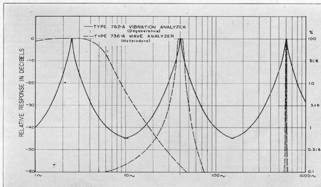
FIGURE 26. Selectivity characteristics of the TYPE 762-A Vibration Analyzer as compared with a typical (TYPE 736-A) heterodyne type of wave analyzer. Of utmost importance is the selectivity curve of the vibration analyzer, which maintains a satisfactory width and shape at both low and high vibration frequencies.
